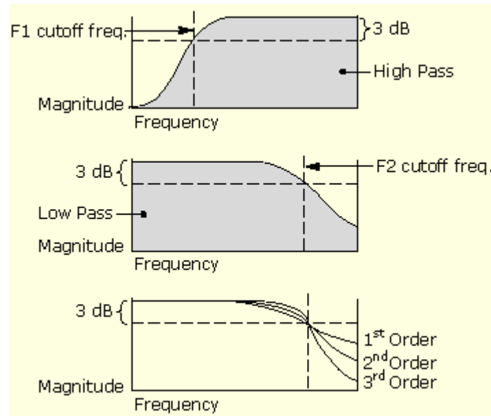
Figure 31: Filter characteristics
